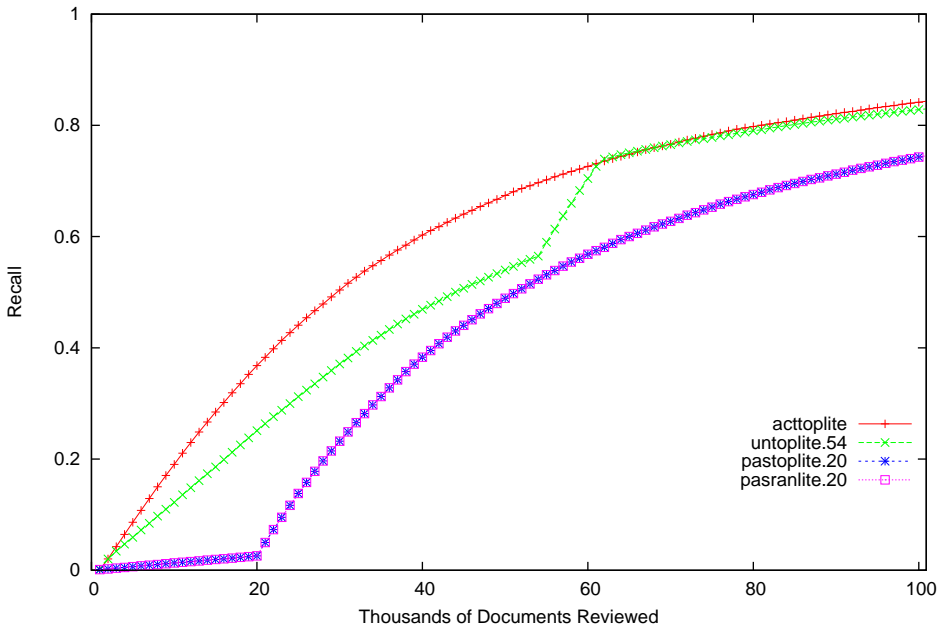
Matter C13 - Recall vs. Documents Reviewed
