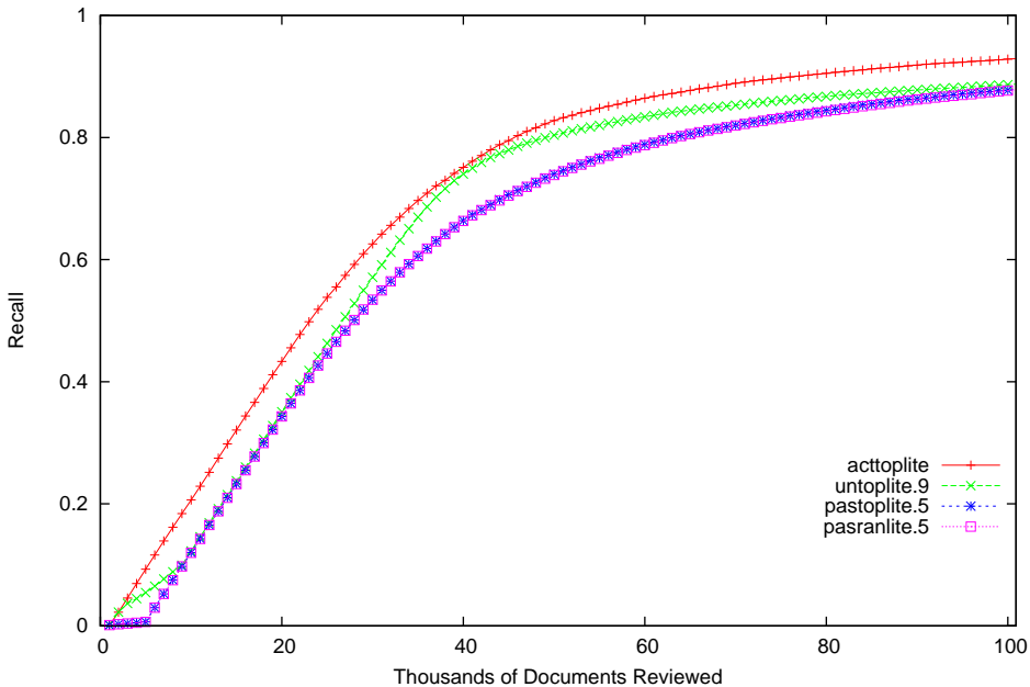
Matter C17 - Recall vs. Documents Reviewed
