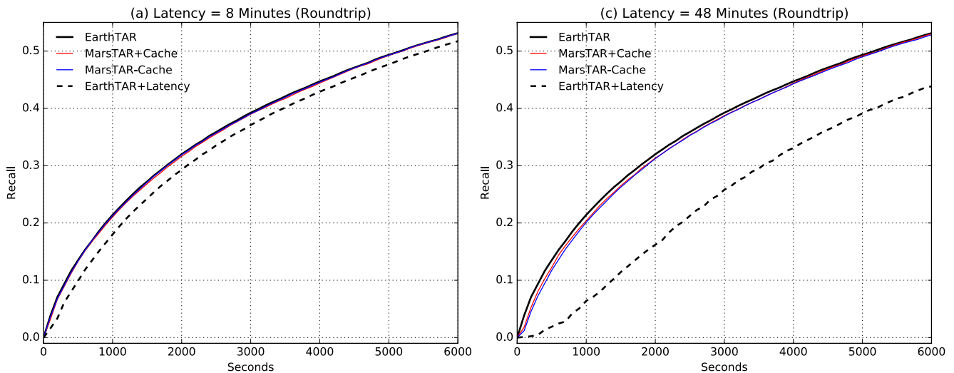
Figure 2: A comparison of the four formulations of AutoTAR with 8-minute (left) and 48-minute (right) roundtrip delays.
