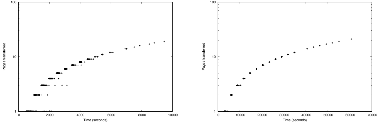
Figure 4: Search sessions on Mars with 8-minute (left) and 48-minute (right) roundtrip delay: Each point represents a single session with no pre-fetching or caching.
