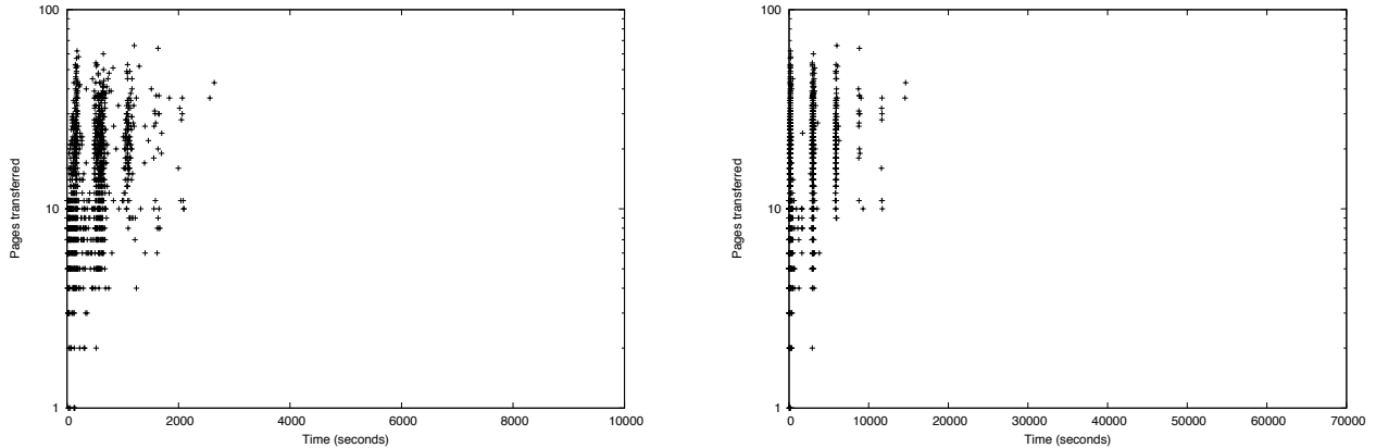
Figure 7: Search sessions on Mars with 8-minute (left) and 48-minute (right) roundtrip delay: Each point represents a single session with SERP pre-fetching and 20% caching. The range of the x axis is the same as in Figures 4 and 5. Pages transferred exclude pages in the cache.
