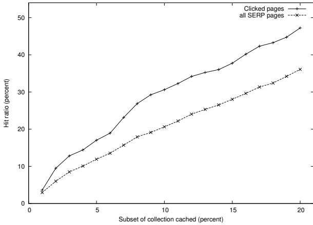
Figure 6: Cache hit ratios for clicked pages and for all SERP result pages.
