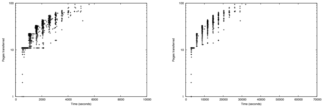
Figure 5: Search sessions on Mars with 8-minute (left) and 48-minute (right) roundtrip delay: Each point represents a single session with SERP pre-fetching.
