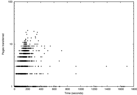
Figure 3: Search sessions on Earth: Each point indicates the pages transferred and total time for a single session.
