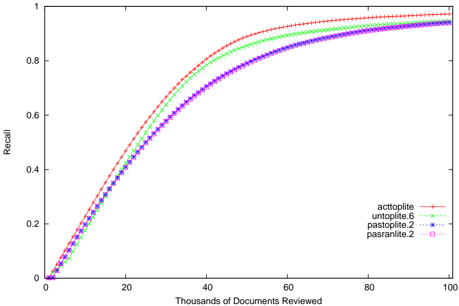
Matter GDIP - Recall vs. Documents Reviewed
